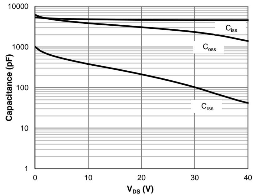
Figure 8: Capacitance Characteristics
