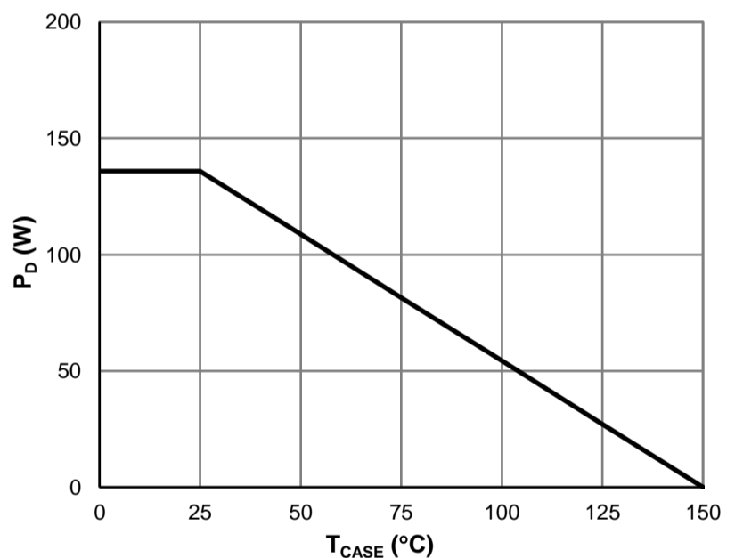
Figure 10: Power De-rating
