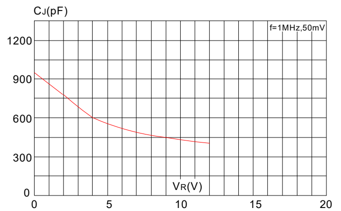
FIG.6: Capacitance vs. reverse voltage
