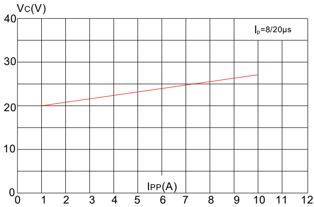
FIG.5: Typical clamping voltage vs. peak pulse current
