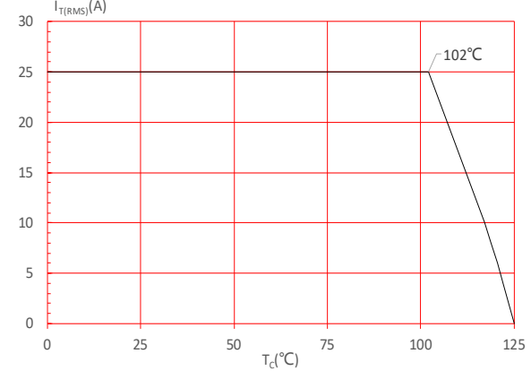
FIG.4: On-state characteristics
