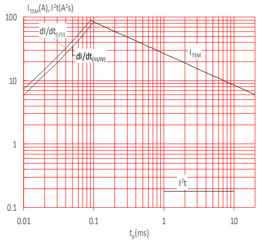
FIG.6: Non-repetitive surge peak on-state current for a sinusoidal pulse with width t_p < 20\text{ms} , and corresponding value of I^2t ( I - II: di/dt < 50\text{A}/\mu\text{s} ; III-IV: di/dt < 20\text{A}/\mu\text{s} )
