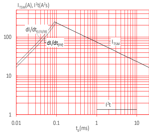
FIG.6: Non-repetitive surge peak on-state current for a sinusoidal pulse with width t_p < 20\text{ms} , and corresponding value of I^2t (I - II -III: di/dt < 50\text{A}/\mu\text{s} ; IV: di/dt < 30\text{A}/\mu\text{s} )
