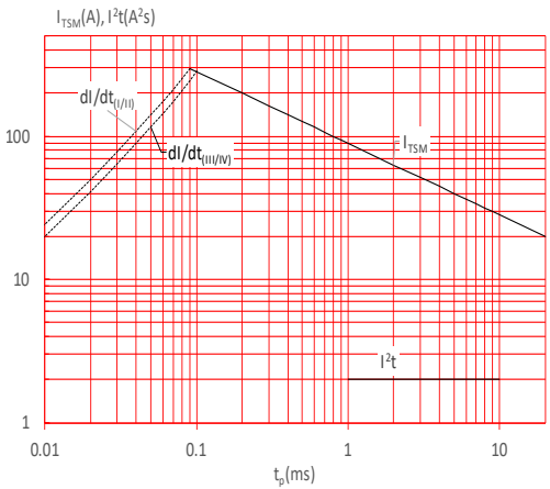
FIG.6: Non-repetitive surge peak on-state current for a sinusoidal pulse with width t_p < 20\text{ms} , and corresponding value of I^2t ( I - II : di/dt < 30\text{A}/\mu\text{s} ; III-IV : di/dt < 20\text{A}/\mu\text{s} )
