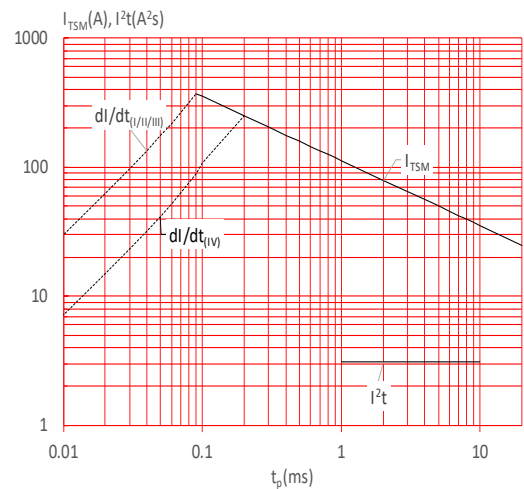
FIG.6: Non-repetitive surge peak on-state current for a sinusoidal pulse with width t_p < 20\text{ms} , and corresponding value of I^2t ( I - II - III: di/dt < 80\text{A}/\mu\text{s} ; IV: di/dt < 40\text{A}/\mu\text{s} )
