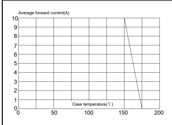
FIG.5 Forward current derating curve (Pin1,3~2)
