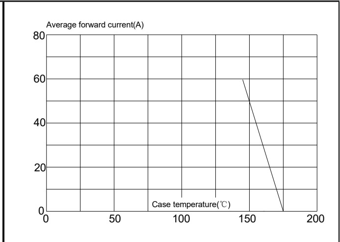
FIG.4: Forward current derating curve (Pin1,3~2)
