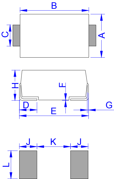
DO-214AA (SMB)
